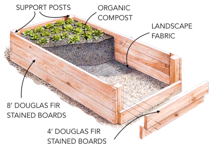
4'x8' RAISED BED
